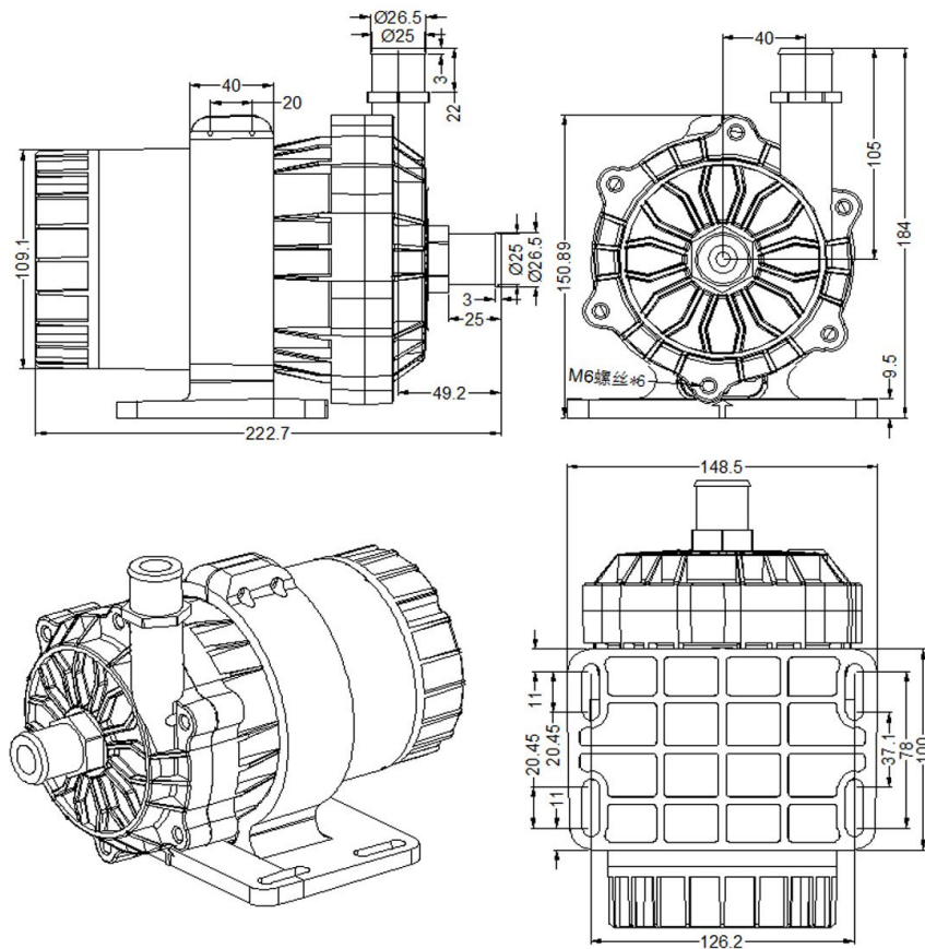
PUMP Body
