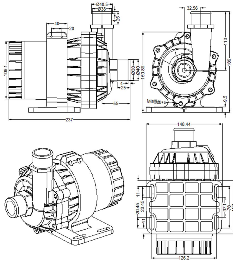
PUMP Body
